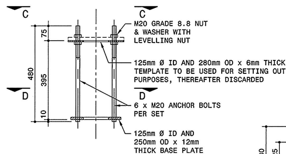
HOLDING DOWN BOLT SET SCALE 1:10
