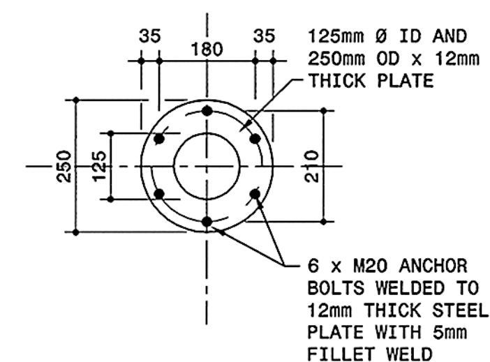
SECTION D-D SCALE 1:10
